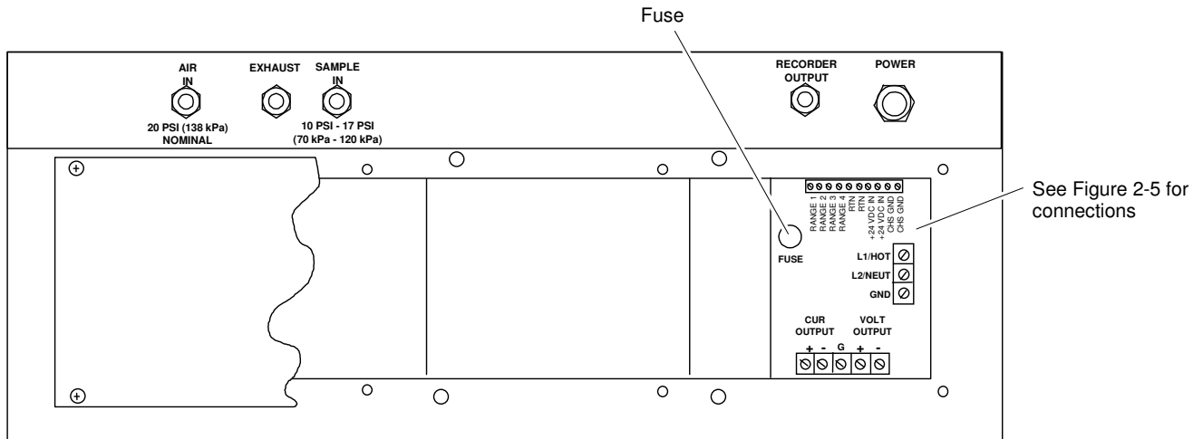
Figure 2-4. Rear View of Model 951C (cover removed)
